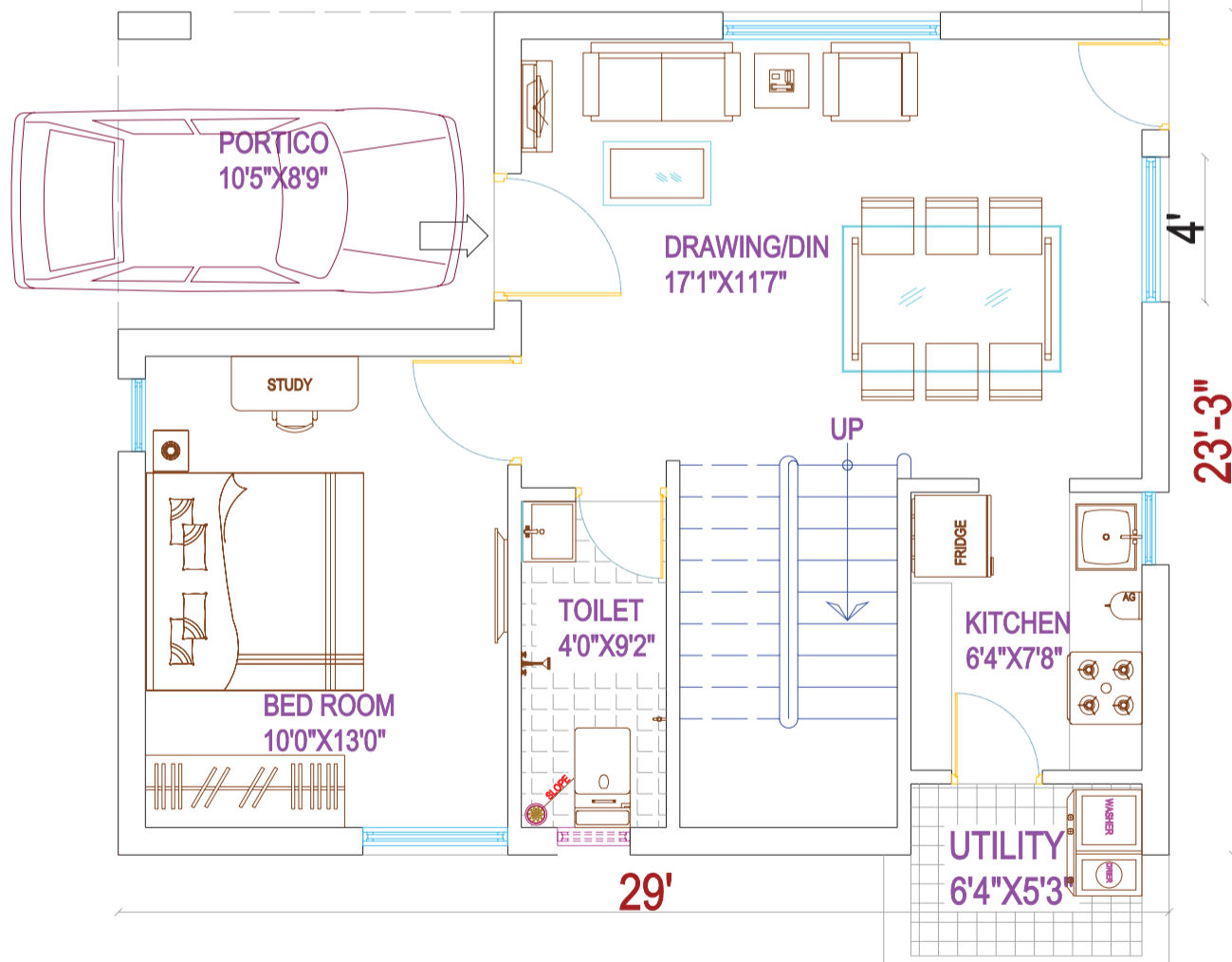
WEST FACING UNIT (GROUND FLOOR PLAN)
