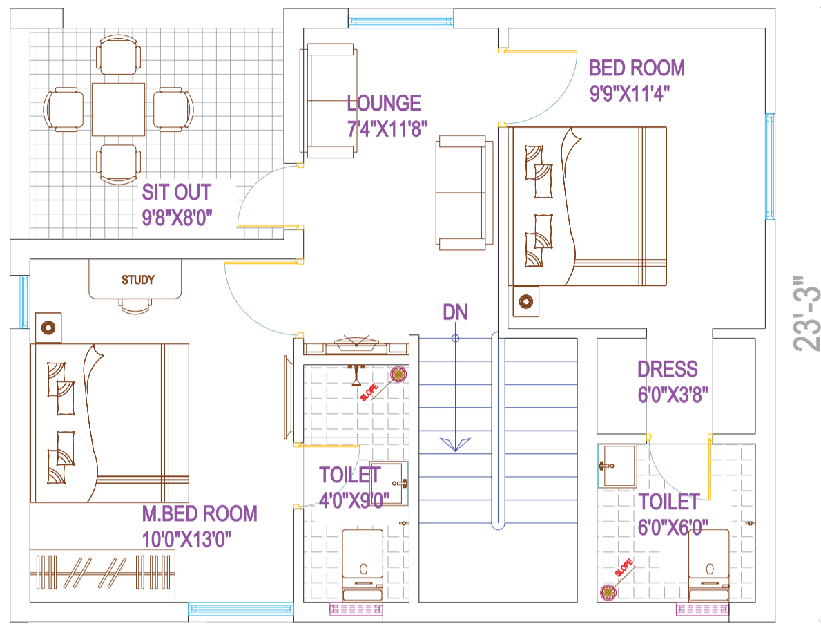
WEST FACING UNIT (FIRST FLOOR PLAN)
