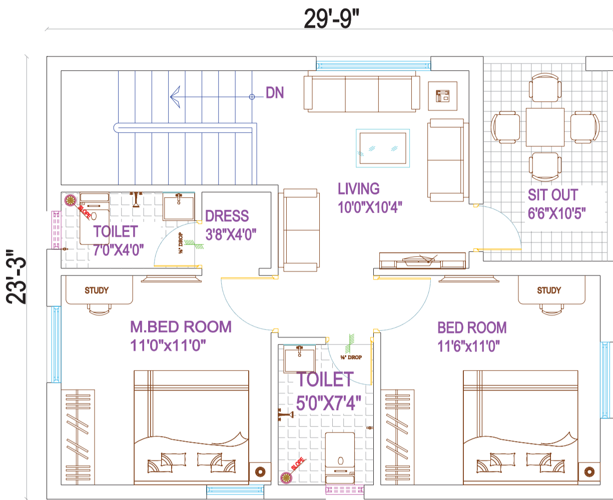
EAST FACING UNIT (FIRST FLOOR PLAN)
