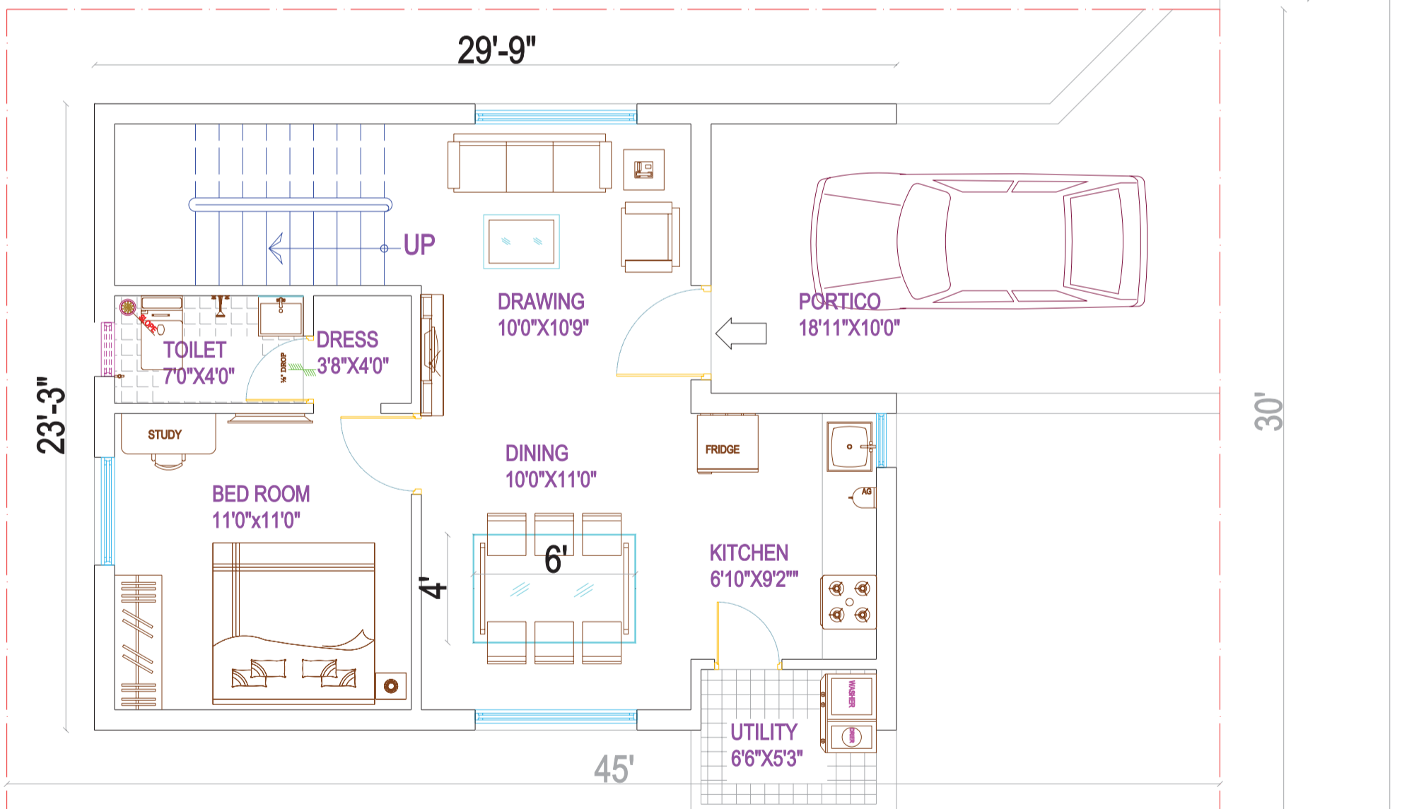
EAST FACING UNIT (GROUND FLOOR PLAN)
